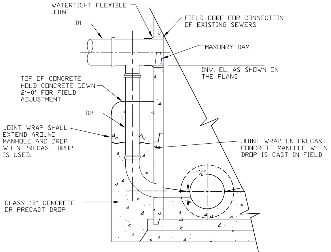
DROP ATTACHMENT NTS
