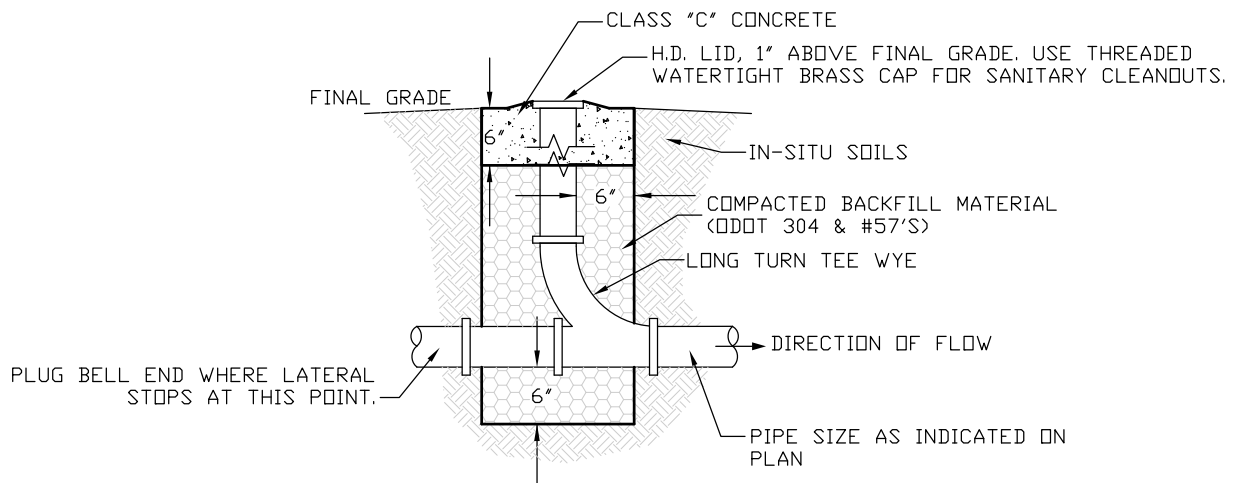
CLEANOUT DETAIL
